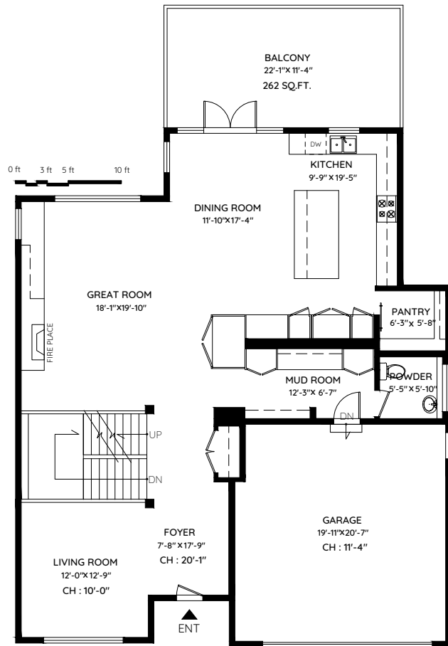
MAIN FLOOR 1,407 SQ.FT. CH: 10'-0"
